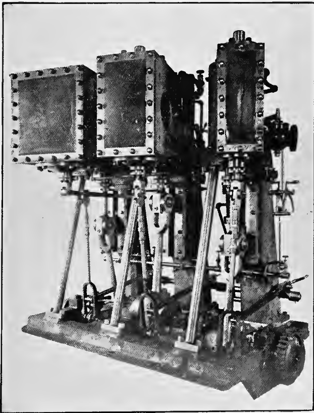
TRIPLE-EXPANSION ENGINE OF THE WOODEN STEAM YACHT CHETOLAH.
